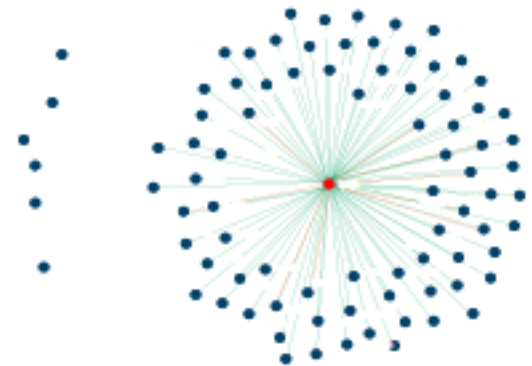
Gene Network
